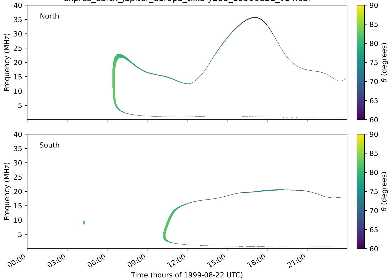
expres_earth_jupiter_europa_txka-y235_19990822_v14.cdf
