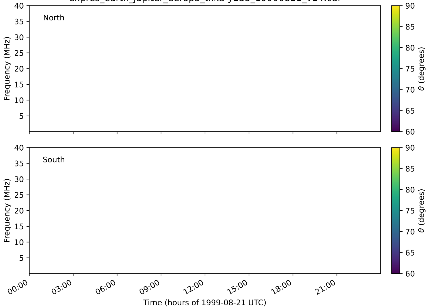
expres_earth_jupiter_europa_txka-y235_19990821_v14.cdf
