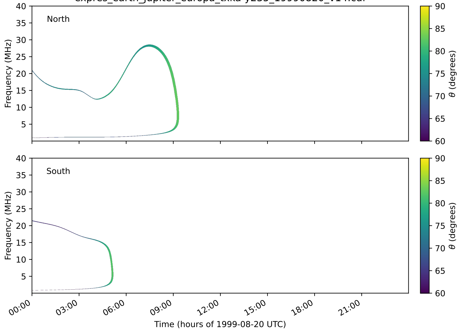
expres_earth_jupiter_europa_txka-y235_19990820_v14.cdf
