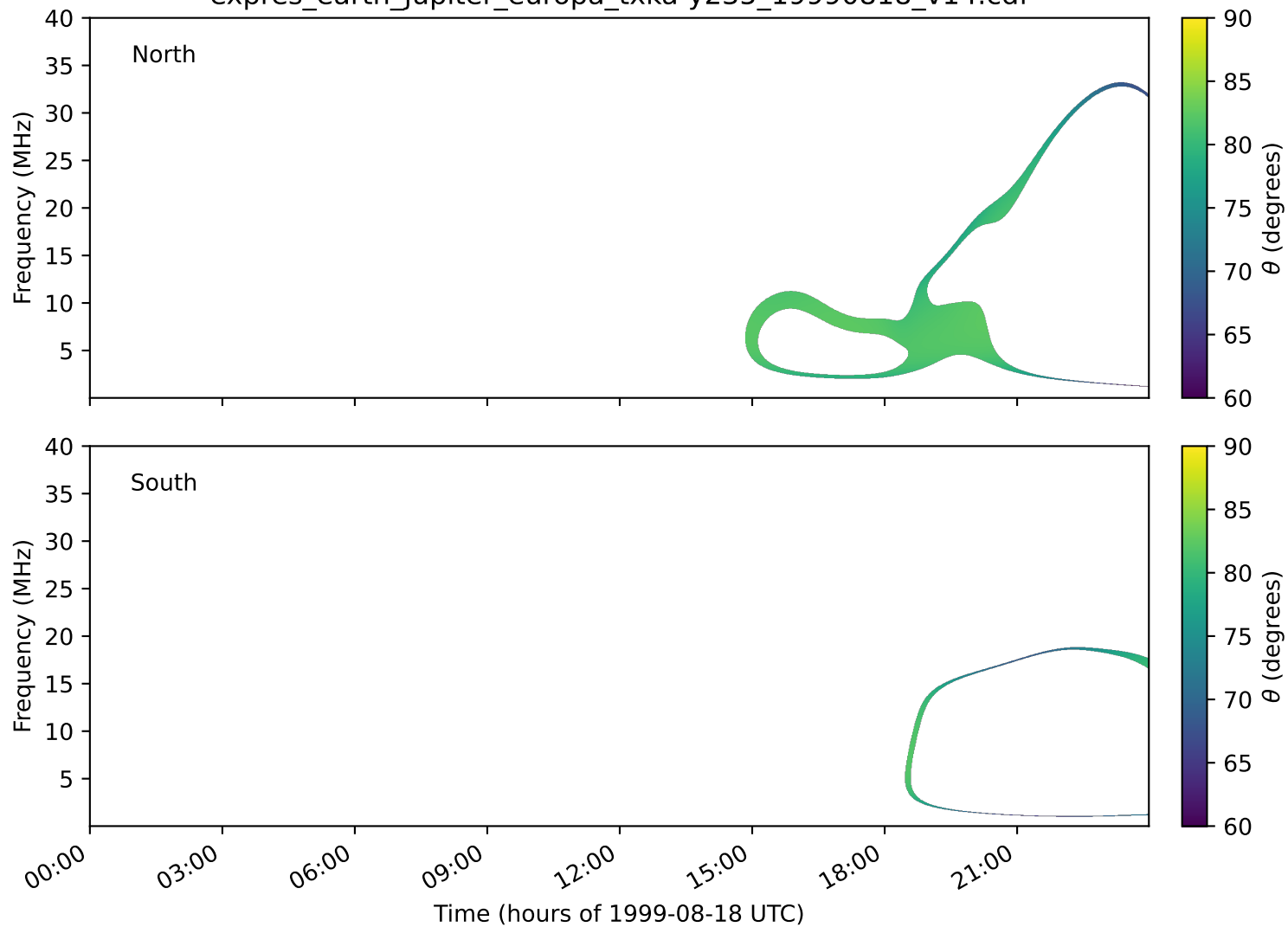
expres_earth_jupiter_europa_txka-y235_19990818_v14.cdf
