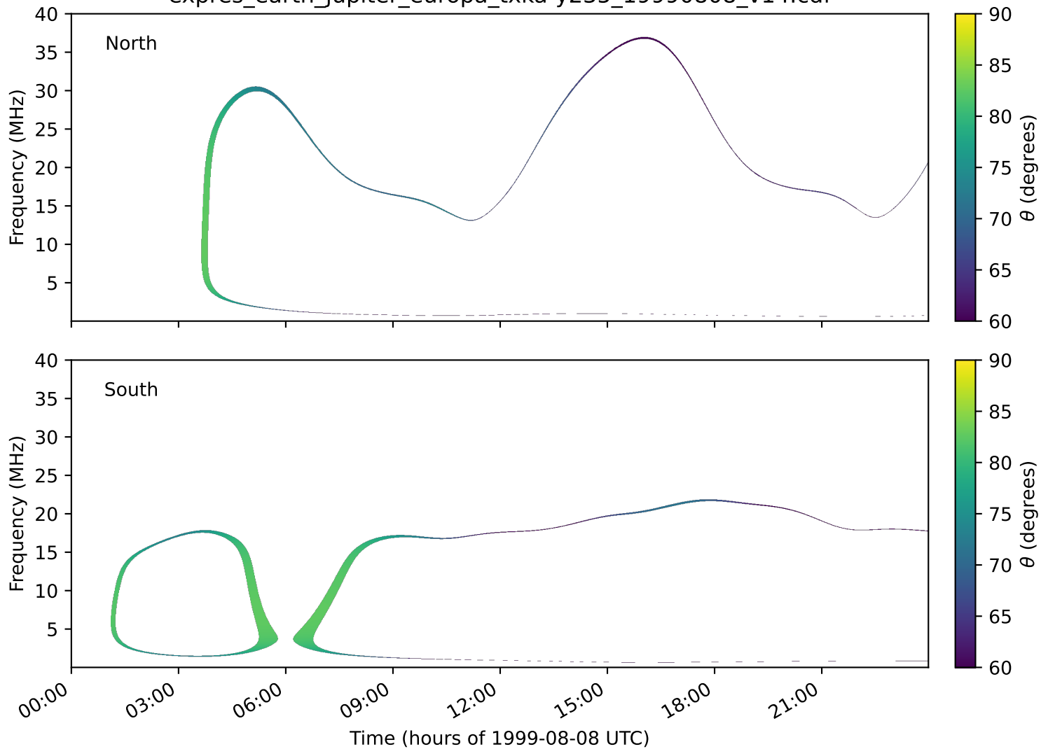
expres_earth_jupiter_europa_txka-y235_19990808_v14.cdf
