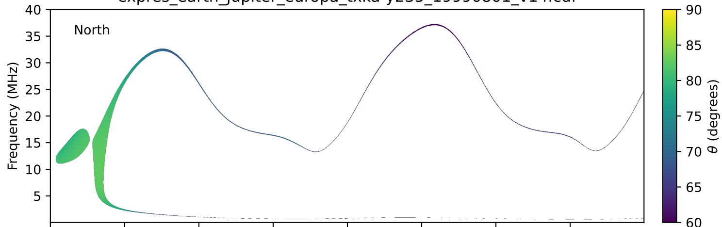
expres_earth_jupiter_europa_txka-y235_19990801_v14.cdf
