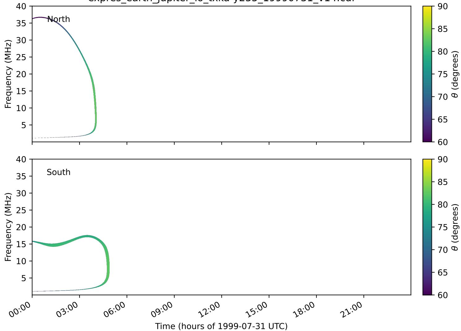
expres_earth_jupiter_io_txka-y235_19990731_v14.cdf
