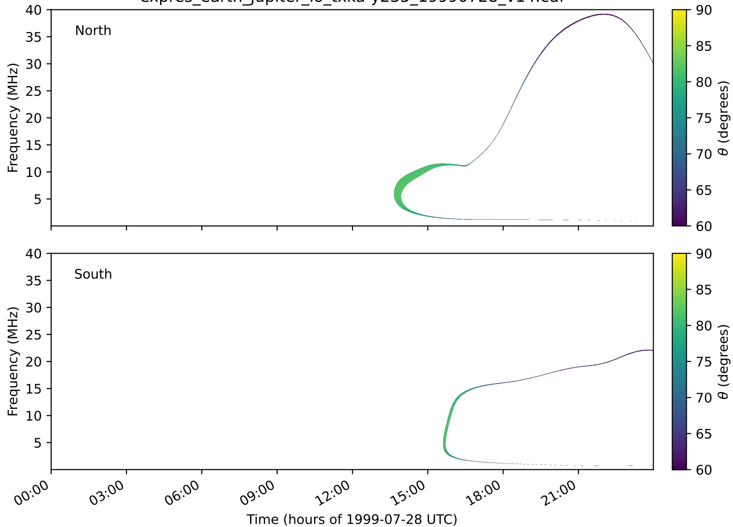
expres_earth_jupiter_io_txka-y235_19990728_v14.cdf
