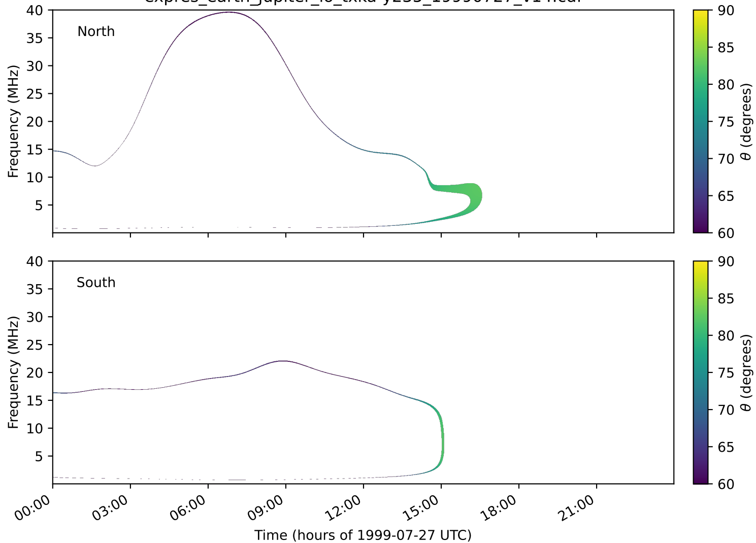
expres_earth_jupiter_io_txka-y235_19990727_v14.cdf
