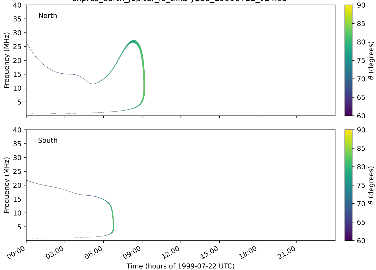
expres_earth_jupiter_io_txka-y235_19990722_v14.cdf
