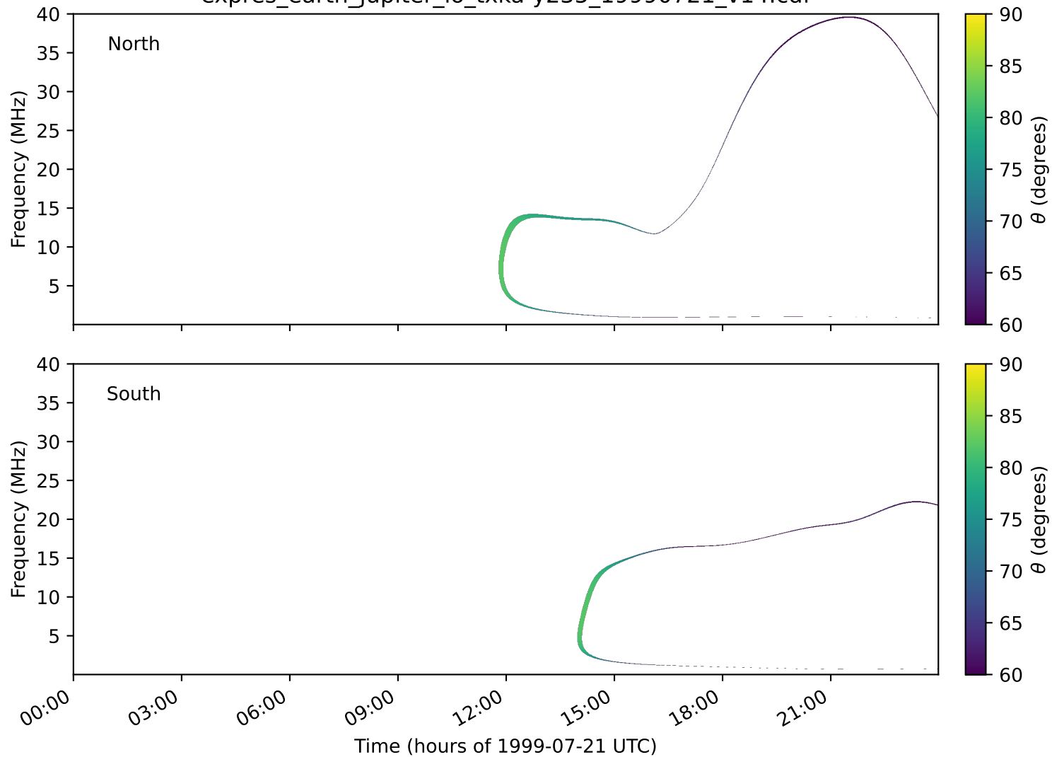
expres_earth_jupiter_io_txka-y235_19990721_v14.cdf
