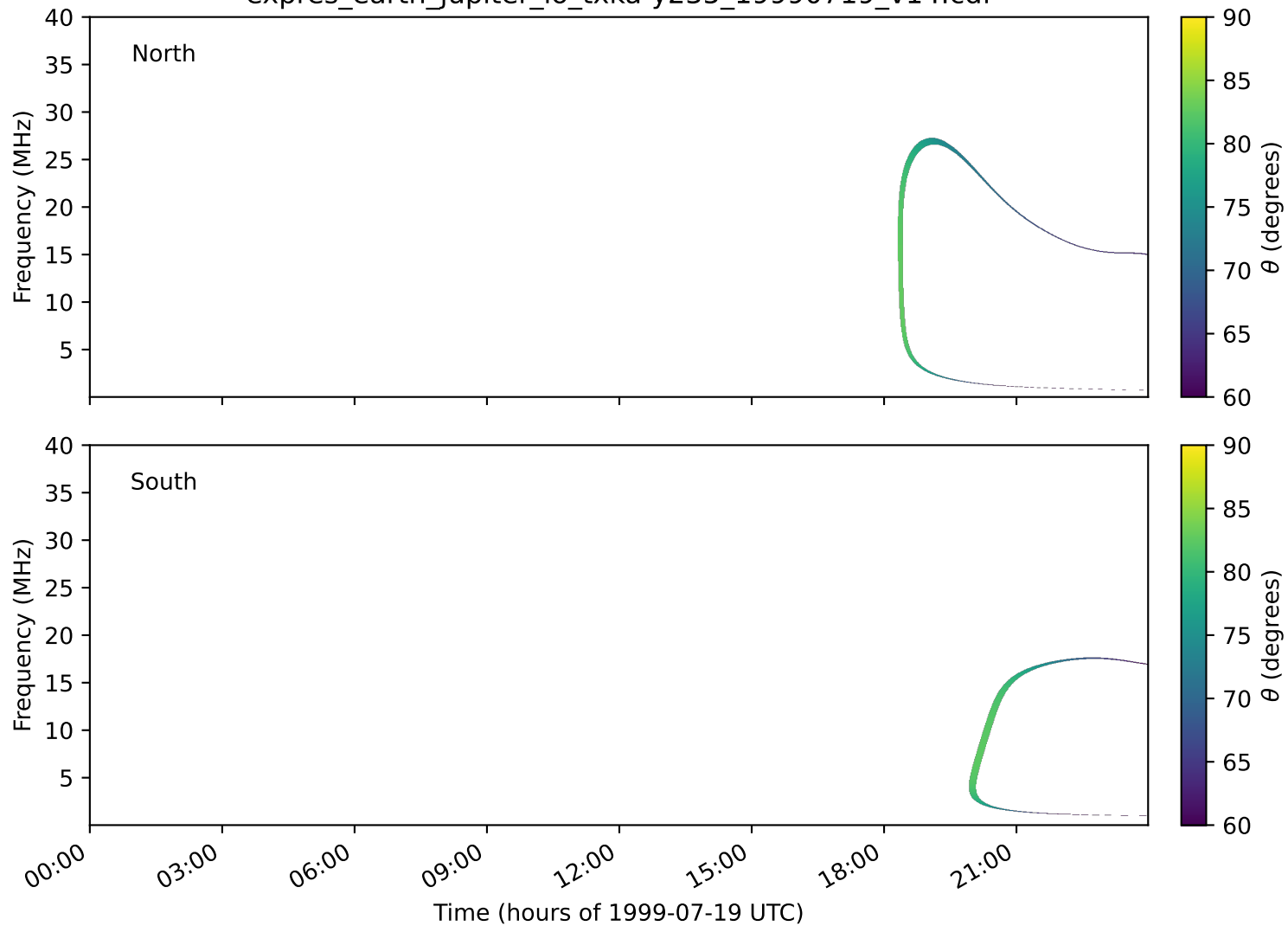
expres_earth_jupiter_io_txka-y235_19990719_v14.cdf
