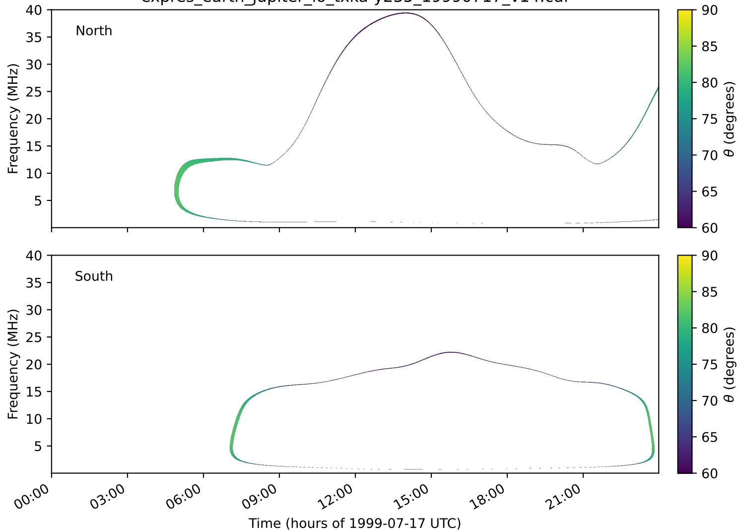
expres_earth_jupiter_io_txka-y235_19990717_v14.cdf
