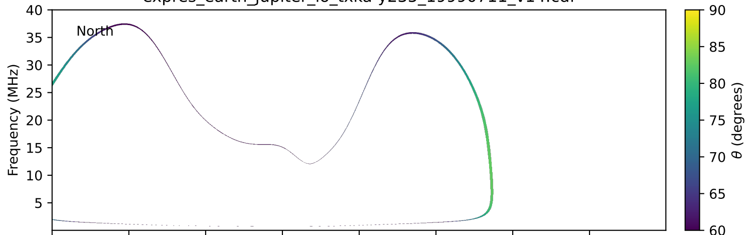
expres_earth_jupiter_io_txka-y235_19990711_v14.cdf
