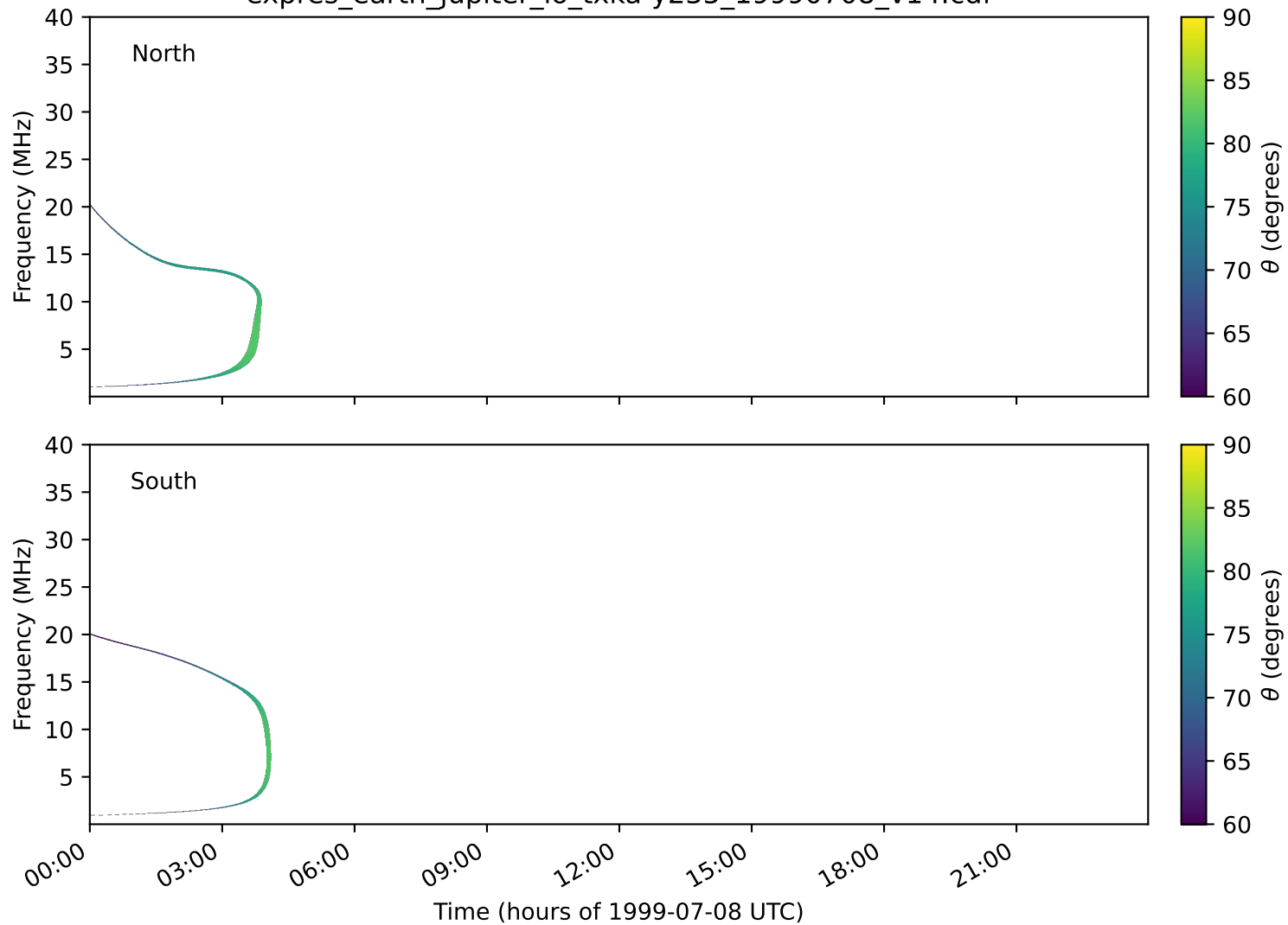
expres_earth_jupiter_io_txka-y235_19990708_v14.cdf
