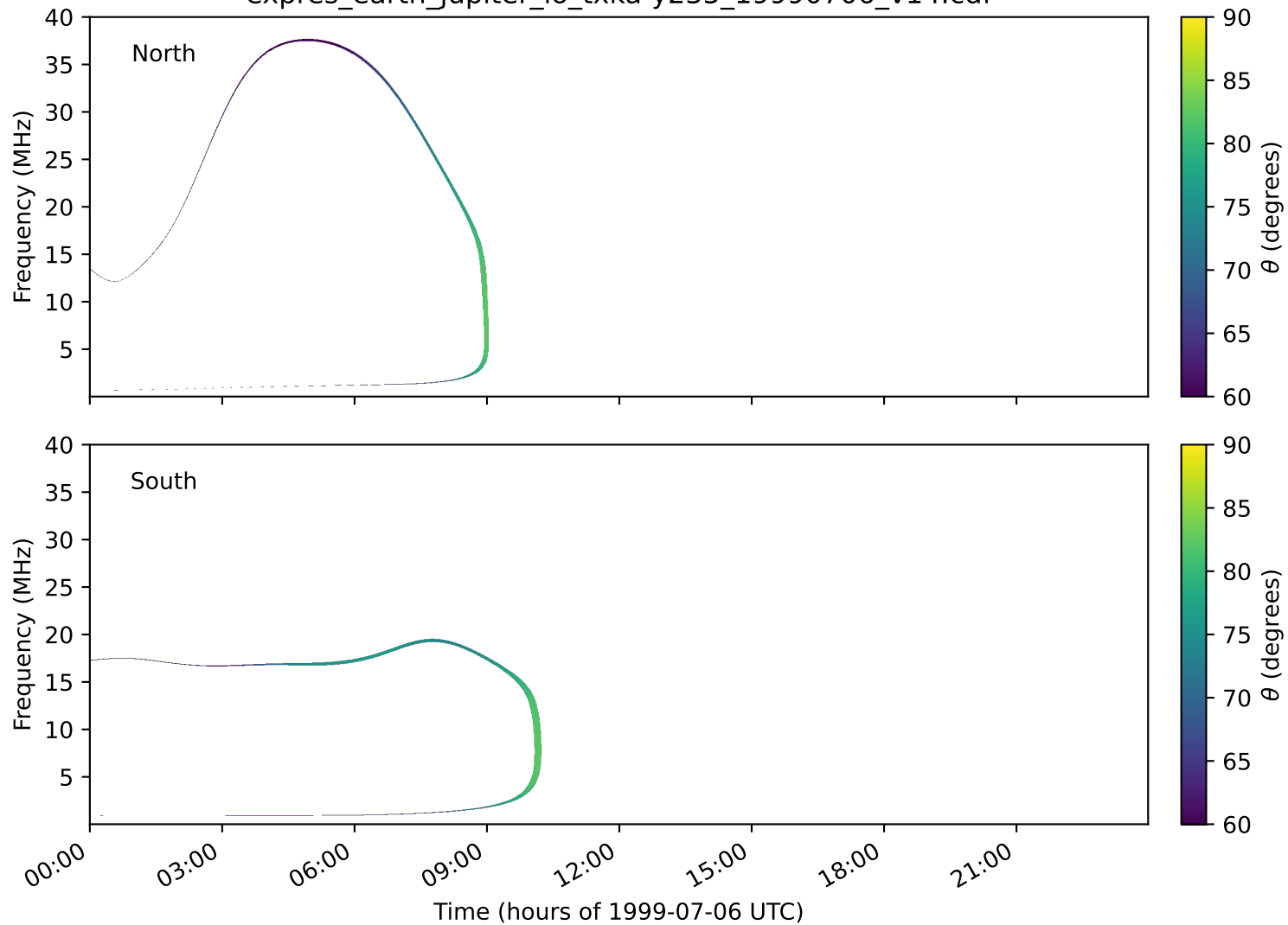
expres_earth_jupiter_io_txka-y235_19990706_v14.cdf
