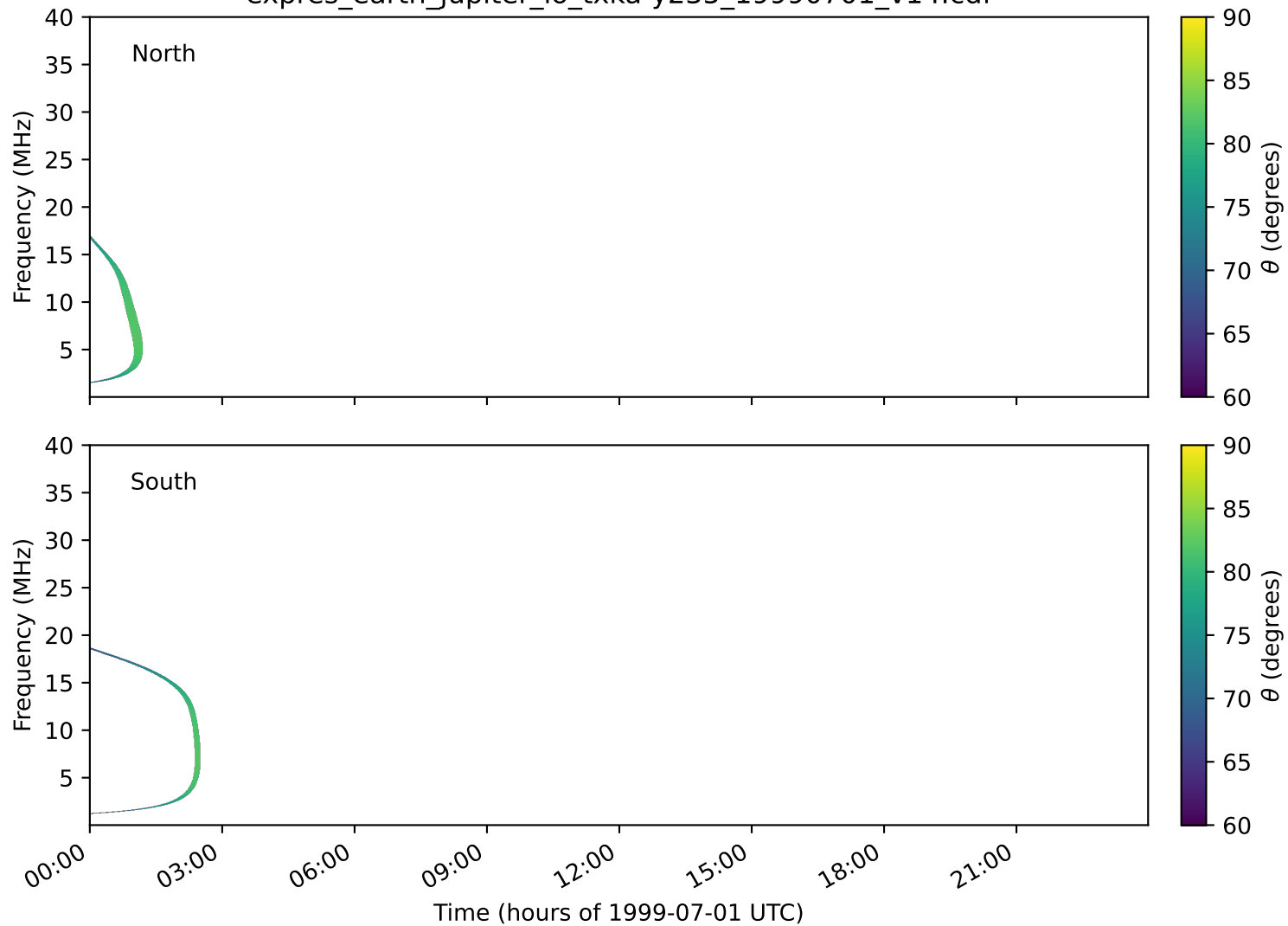
expres_earth_jupiter_io_txka-y235_19990701_v14.cdf
