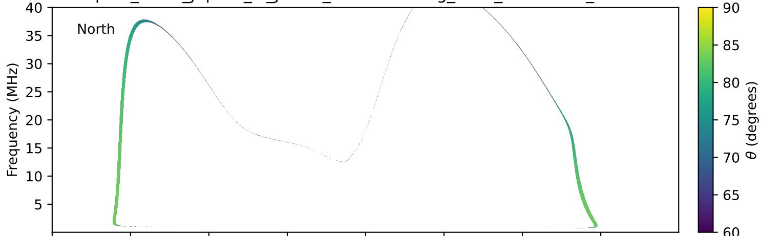
expres_earth_jupiter_io_jrm09_lossc-wid1deg_3kev_19990725_v11.cdf
