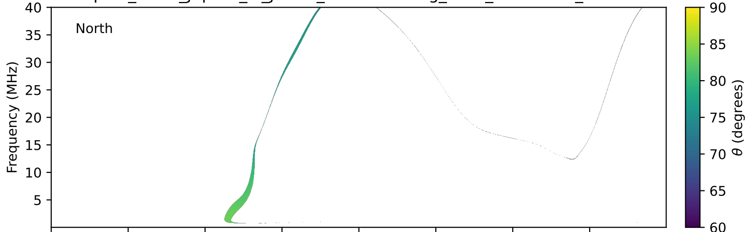
expres_earth_jupiter_io_jrm09_lossc-wid1deg_3kev_19990723_v11.cdf
