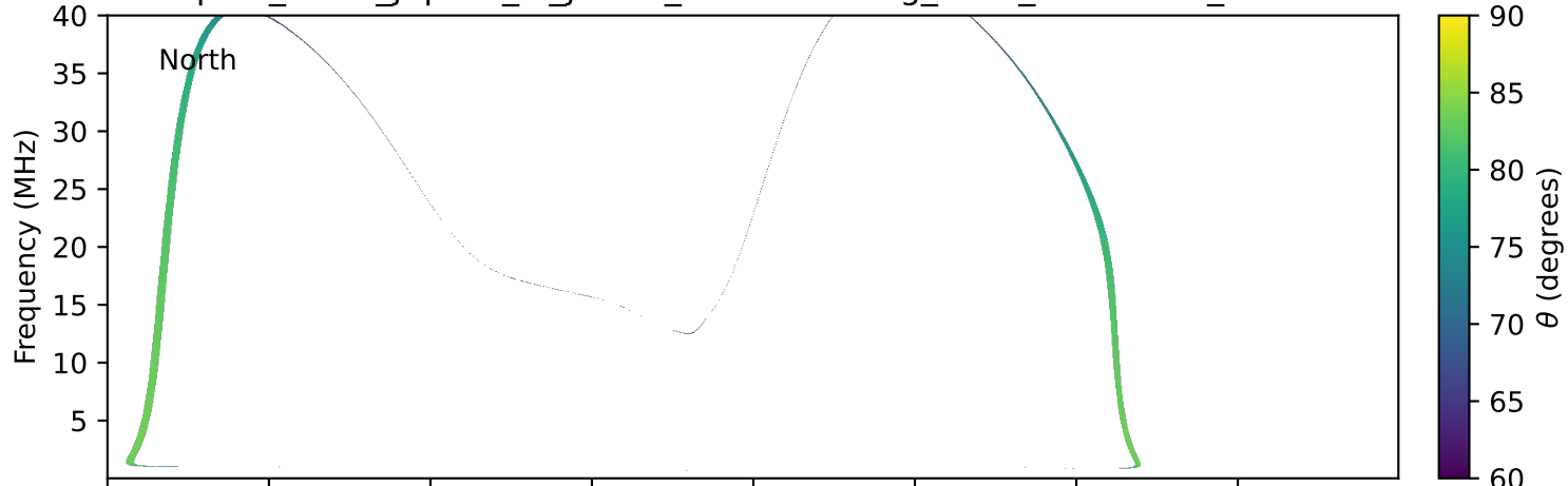
expres_earth_jupiter_io_jrm09_lossc-wid1deg_3kev_19990718_v11.cdf
