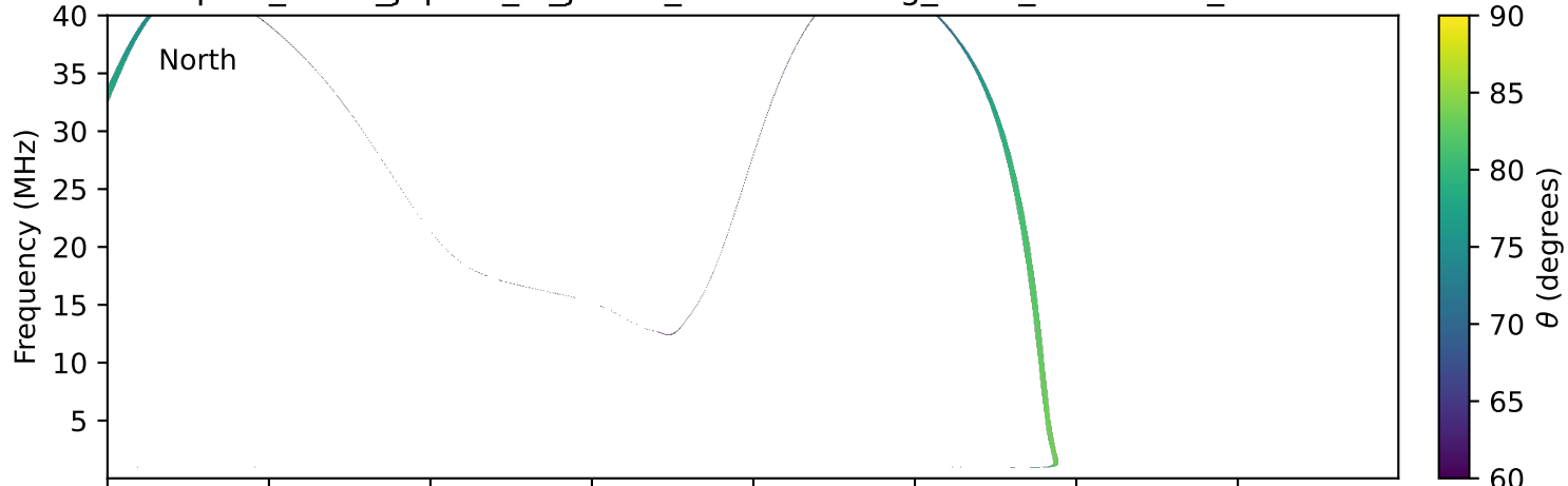
expres_earth_jupiter_io_jrm09_lossc-wid1deg_3kev_19990711_v11.cdf
