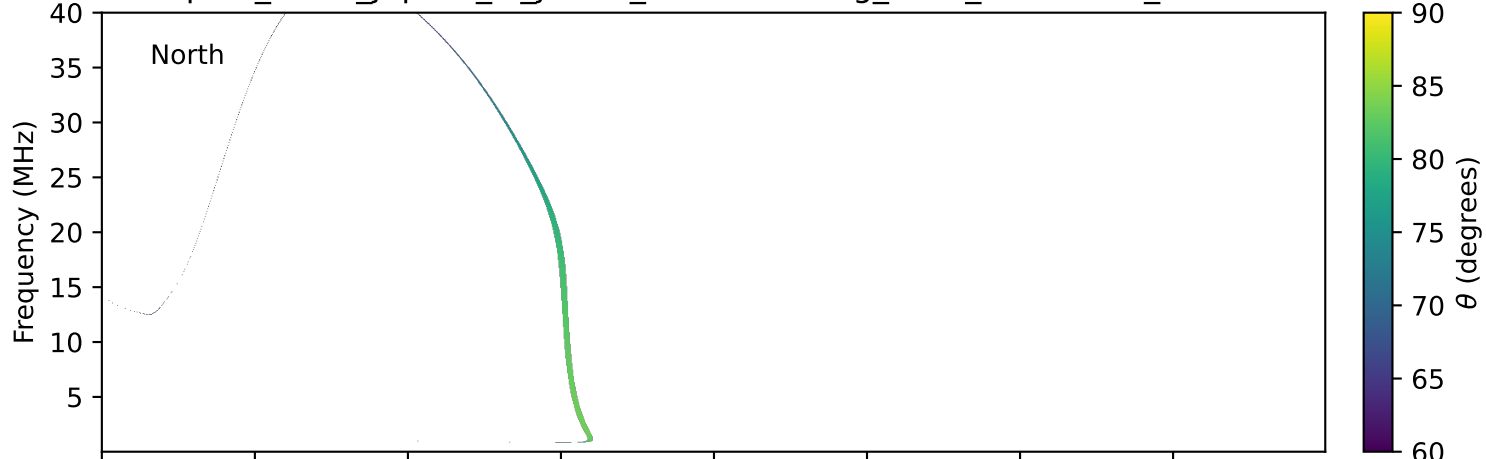
expres_earth_jupiter_io_jrm09_lossc-wid1deg_3kev_19990706_v11.cdf
