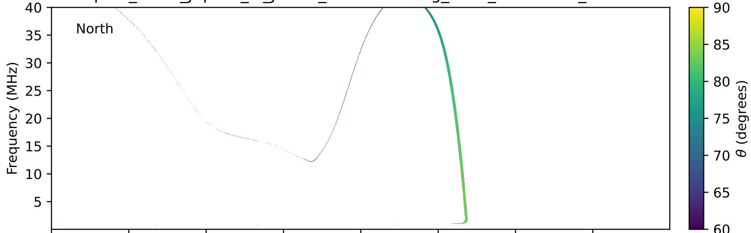
expres_earth_jupiter_io_jrm09_lossc-wid1deg_3kev_19990704_v11.cdf
