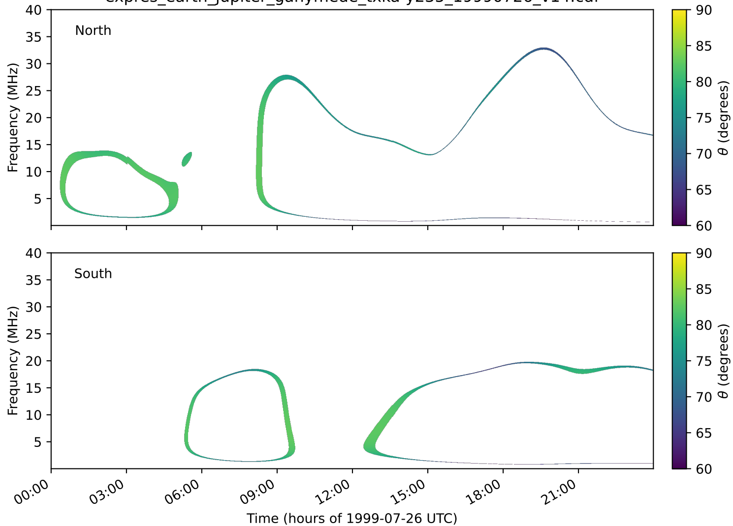
expres_earth_jupiter_ganymede_txka-y235_19990726_v14.cdf
