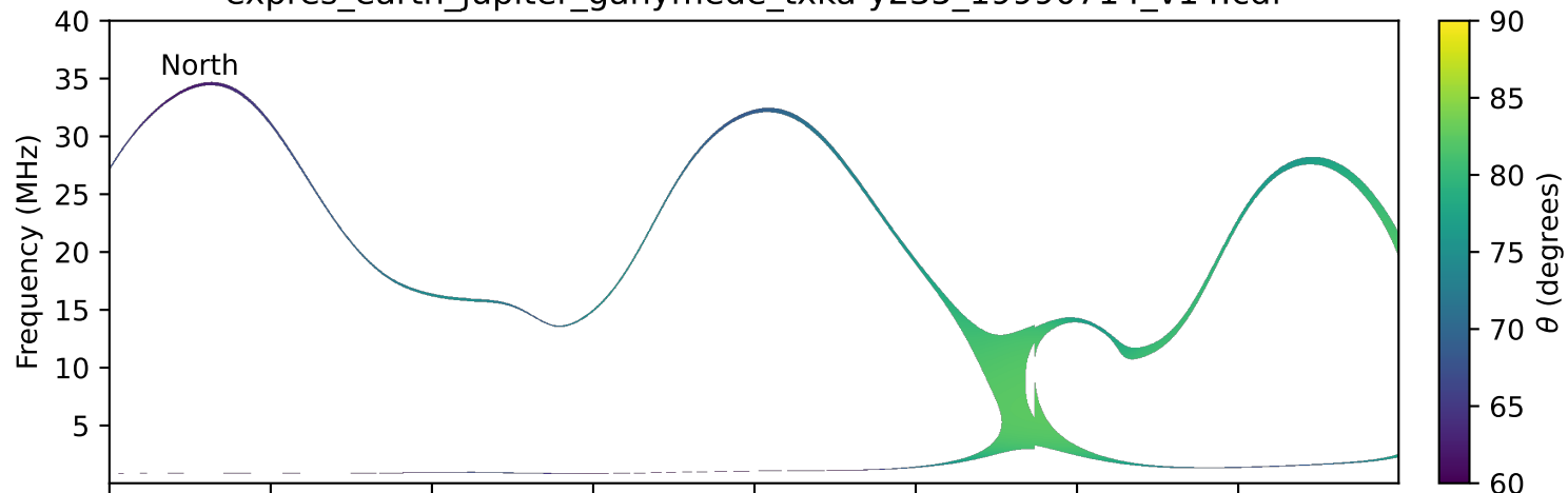
expres_earth_jupiter_ganymede_txka-y235_19990714_v14.cdf
