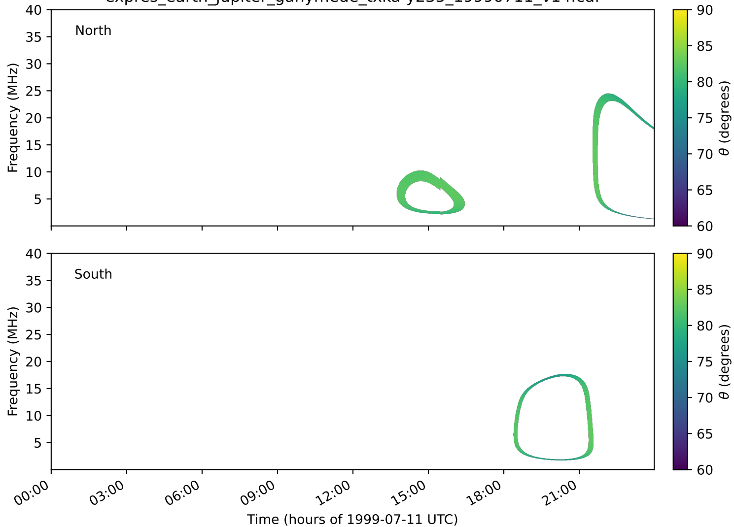
expres_earth_jupiter_ganymede_txka-y235_19990711_v14.cdf
