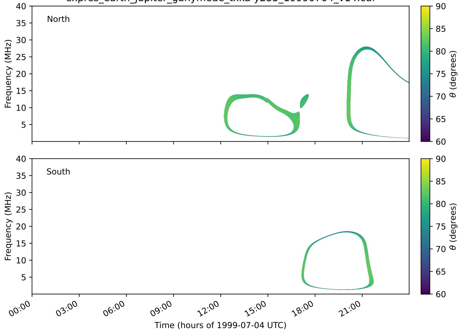
expres_earth_jupiter_ganymede_txka-y235_19990704_v14.cdf
