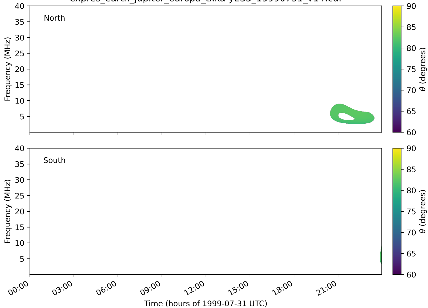
expres_earth_jupiter_europa_txka-y235_19990731_v14.cdf
