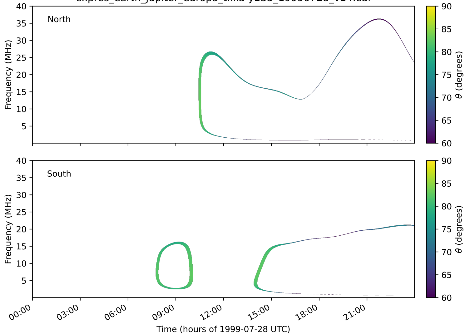
expres_earth_jupiter_europa_txka-y235_19990728_v14.cdf
