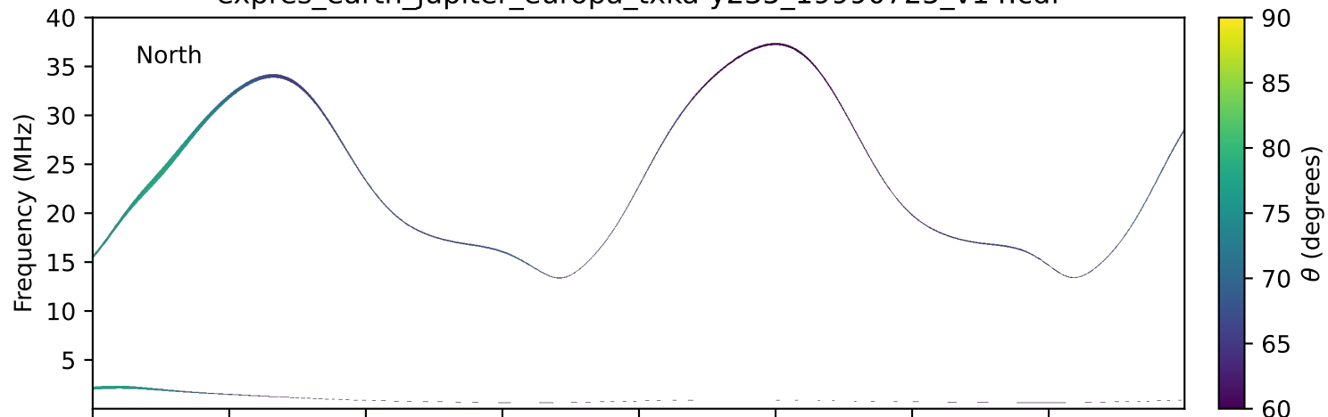
expres_earth_jupiter_europa_txka-y235_19990725_v14.cdf
