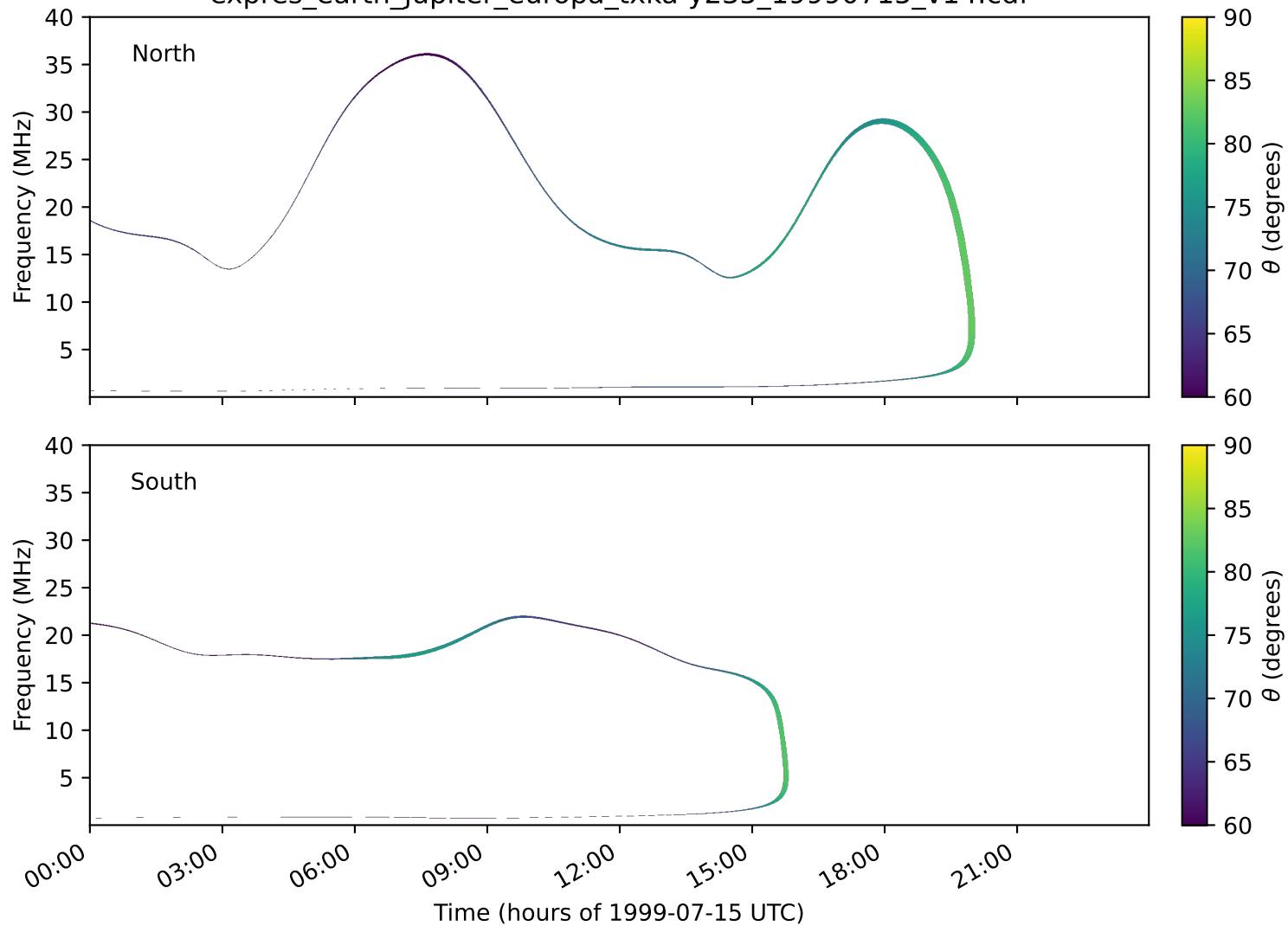
expres_earth_jupiter_europa_txka-y235_19990715_v14.cdf
