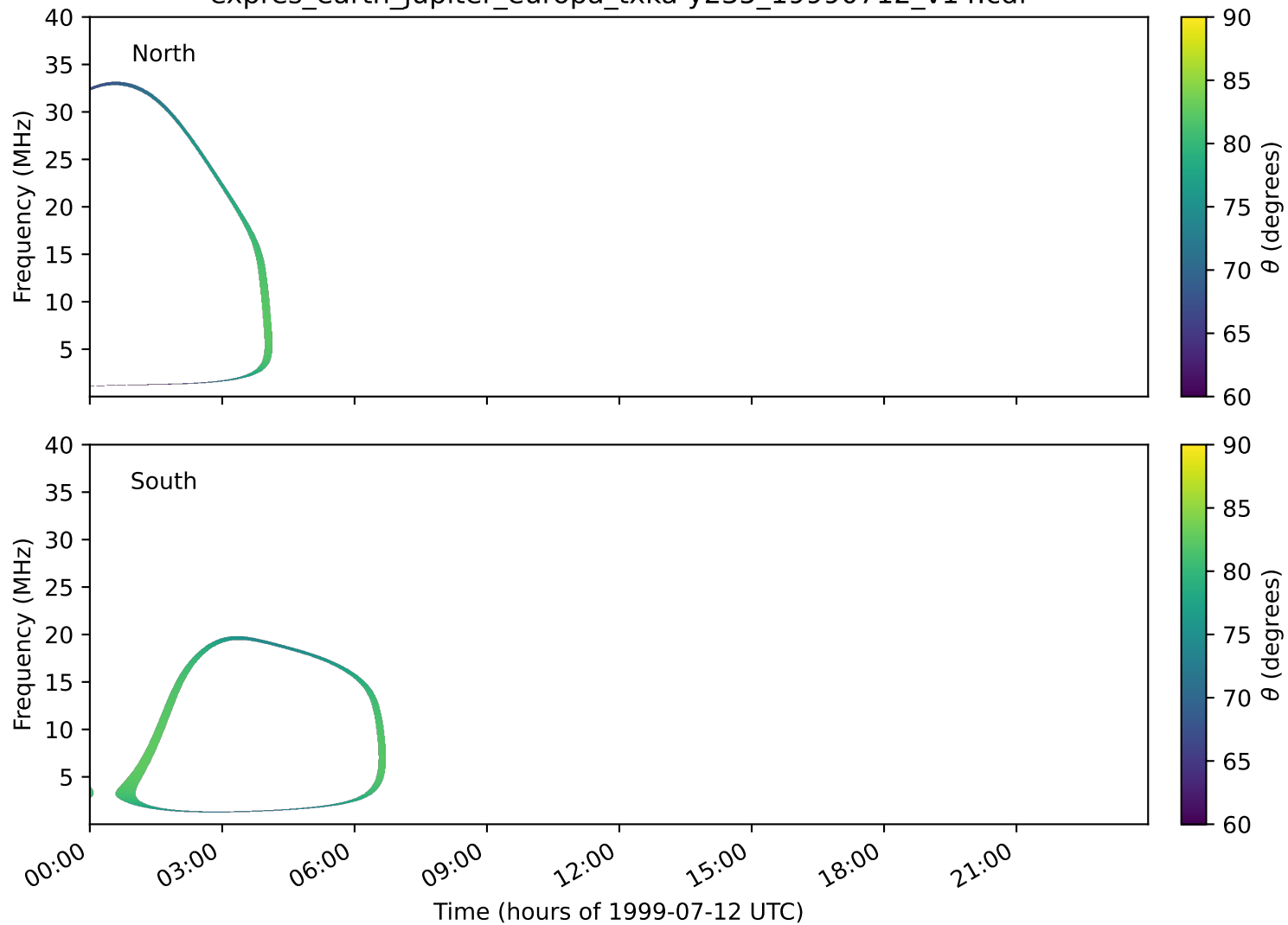
expres_earth_jupiter_europa_txka-y235_19990712_v14.cdf
