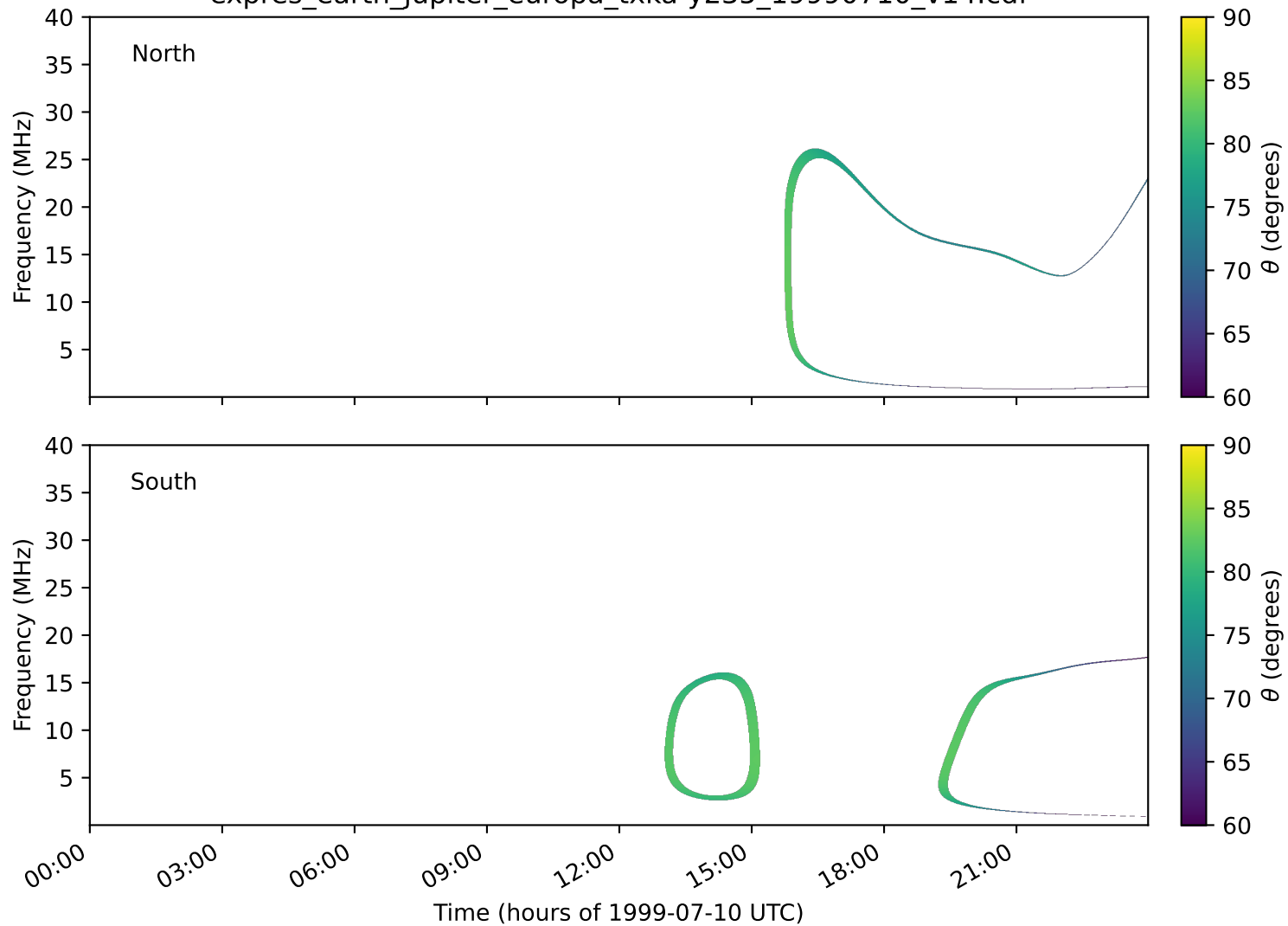
expres_earth_jupiter_europa_txka-y235_19990710_v14.cdf
