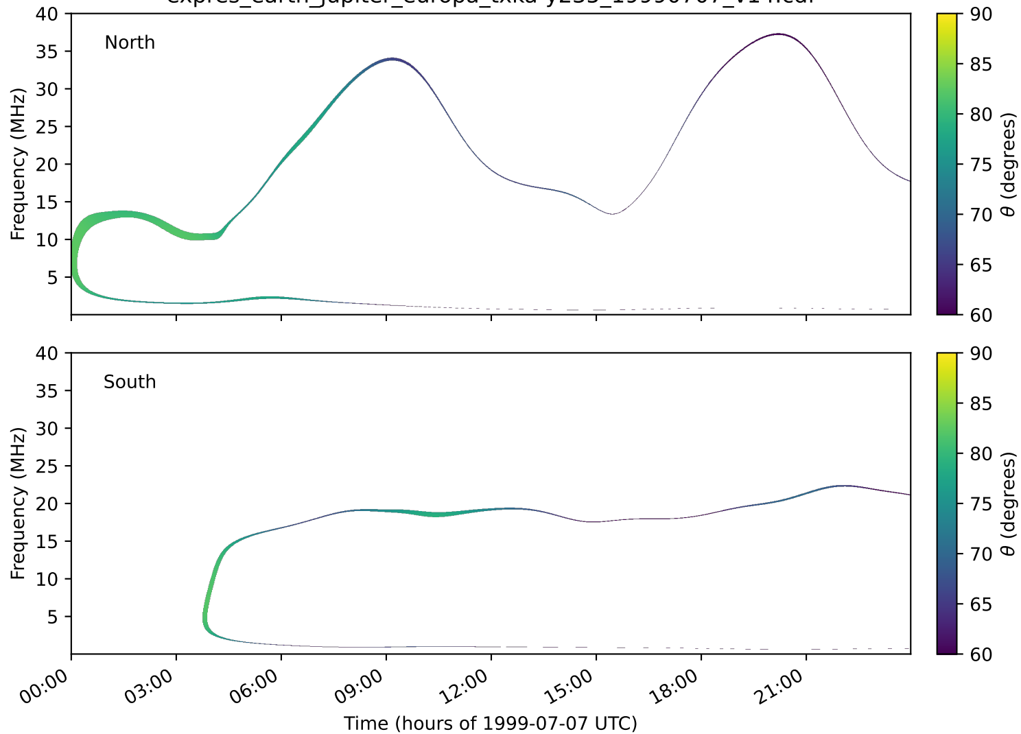
expres_earth_jupiter_europa_txka-y235_19990707_v14.cdf
