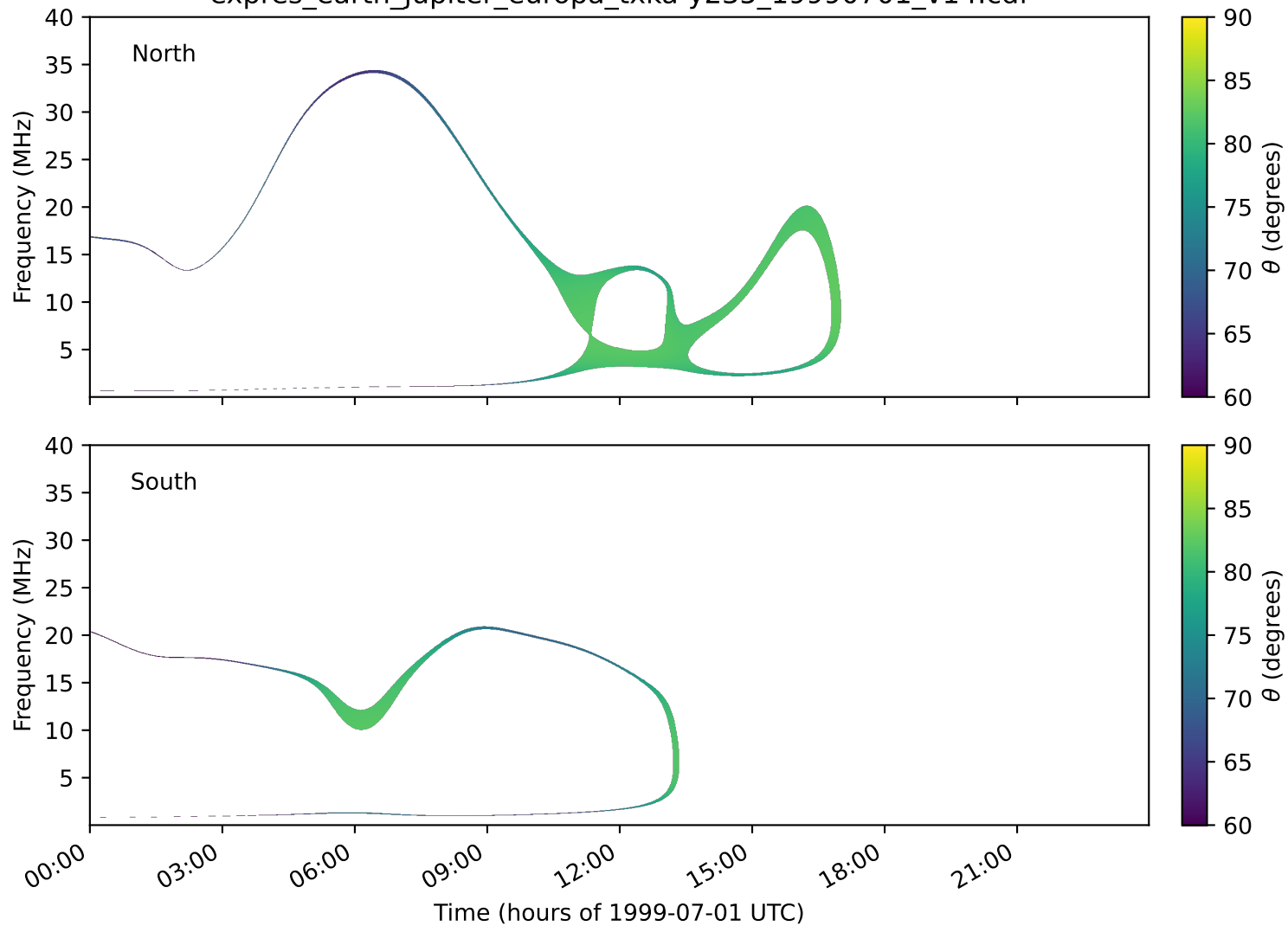
expres_earth_jupiter_europa_txka-y235_19990701_v14.cdf
