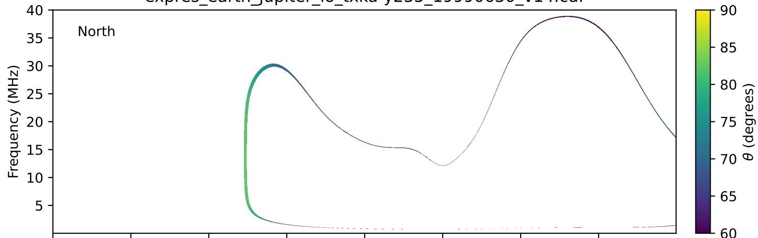
expres_earth_jupiter_io_txka-y235_19990630_v14.cdf
