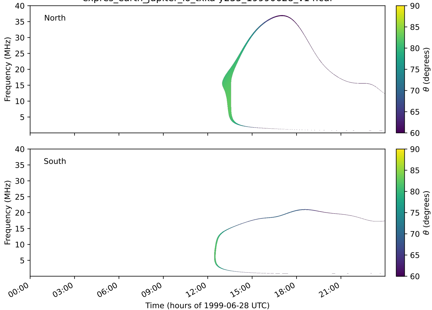
expres_earth_jupiter_io_txka-y235_19990628_v14.cdf
