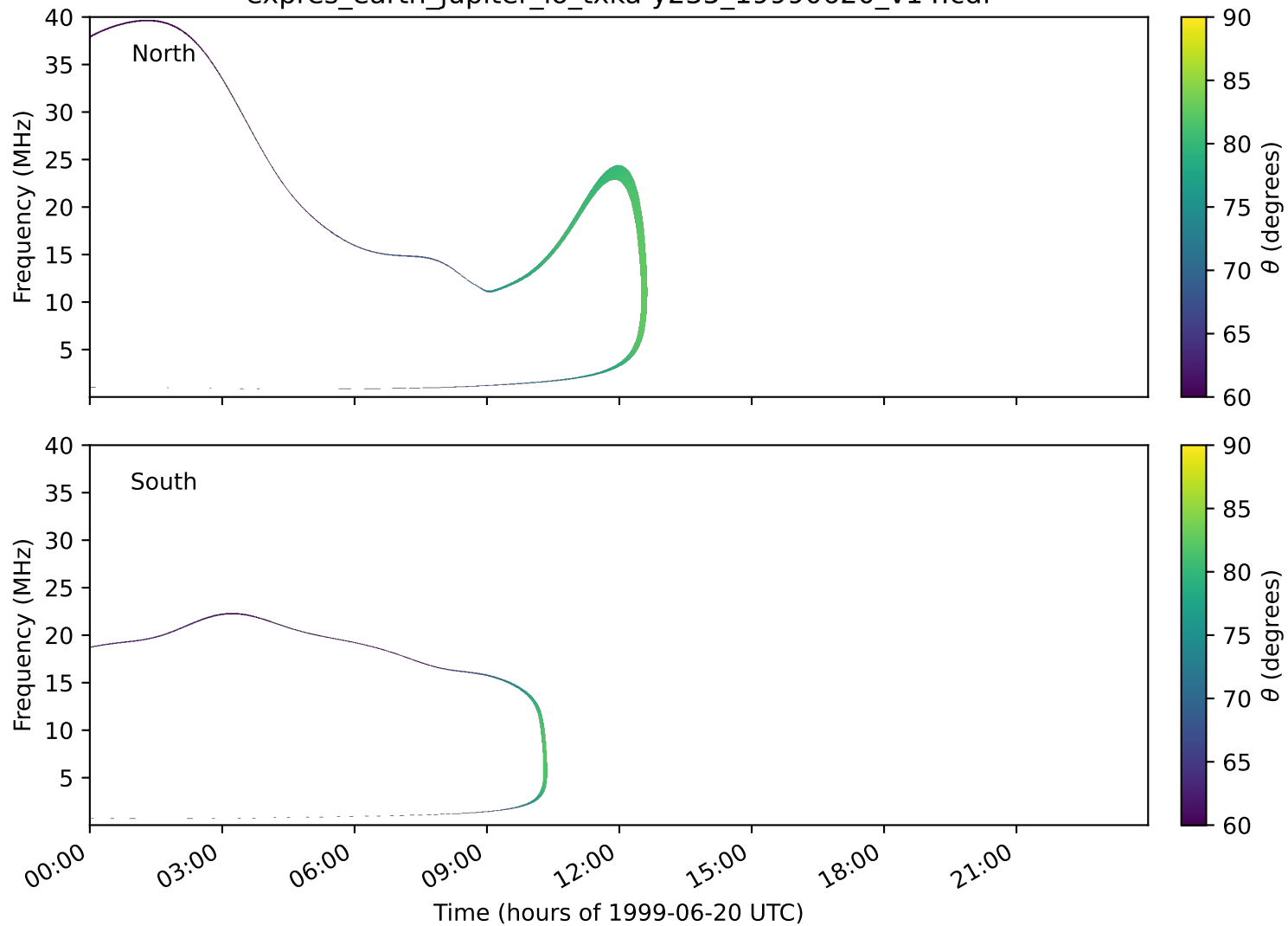
expres_earth_jupiter_io_txka-y235_19990620_v14.cdf
