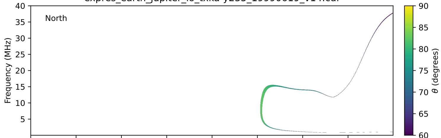
expres_earth_jupiter_io_txka-y235_19990619_v14.cdf
