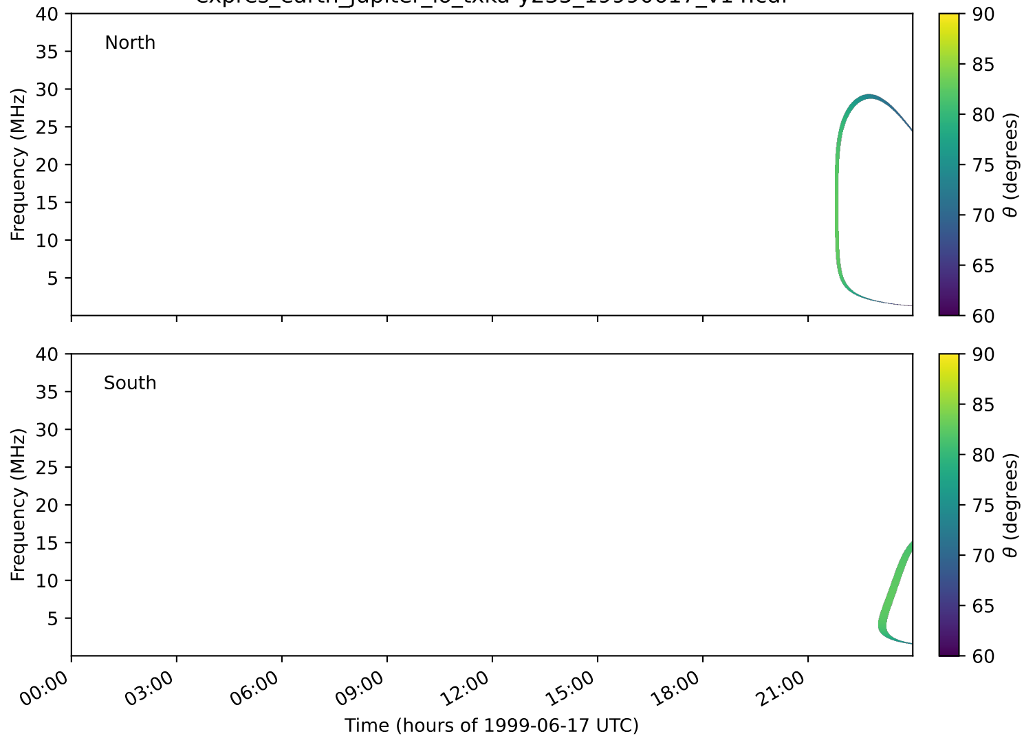
expres_earth_jupiter_io_txka-y235_19990617_v14.cdf
