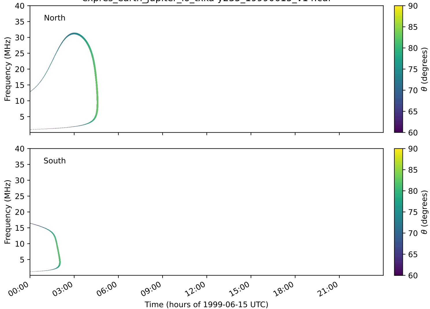
expres_earth_jupiter_io_txka-y235_19990615_v14.cdf
