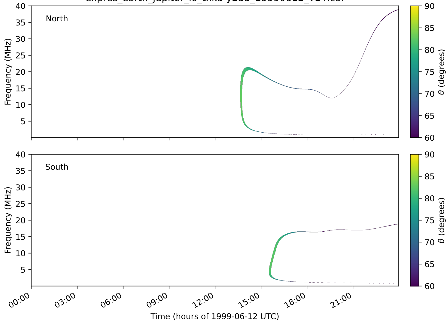
expres_earth_jupiter_io_txka-y235_19990612_v14.cdf
