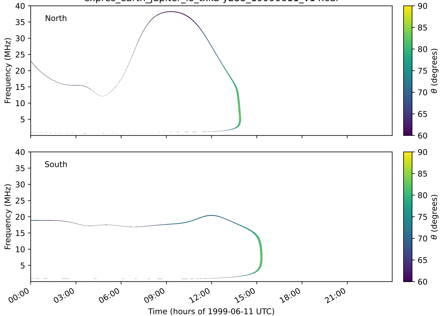
expres_earth_jupiter_io_txka-y235_19990611_v14.cdf
