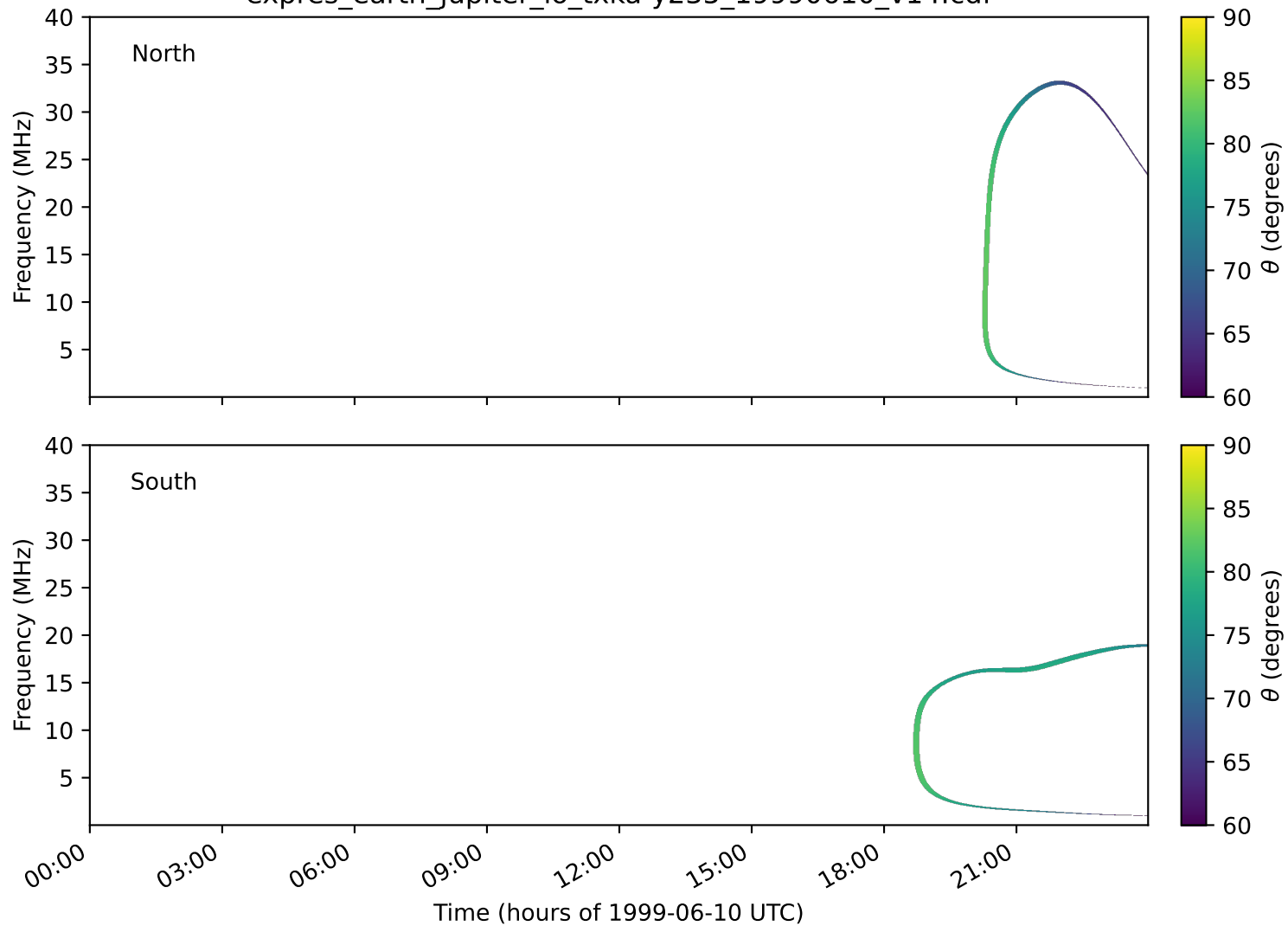
expres_earth_jupiter_io_txka-y235_19990610_v14.cdf
