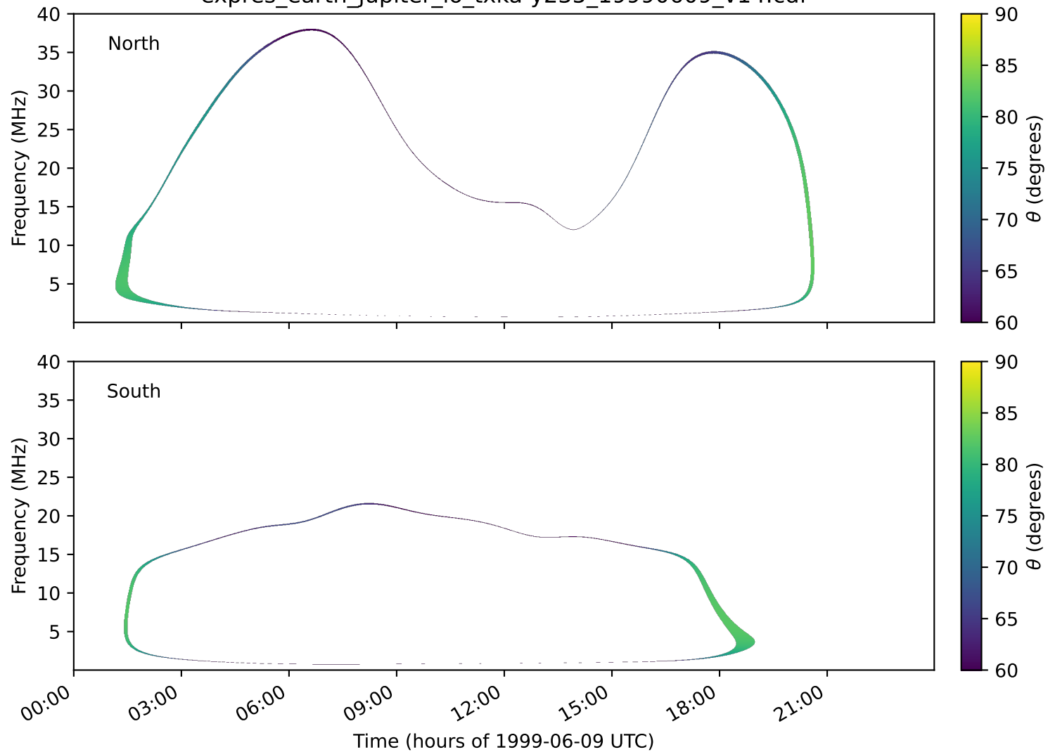
expres_earth_jupiter_io_txka-y235_19990609_v14.cdf
