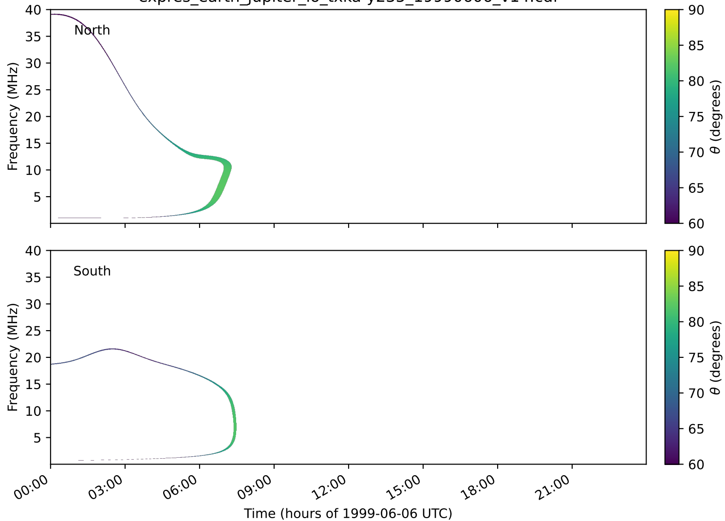
expres_earth_jupiter_io_txka-y235_19990606_v14.cdf
