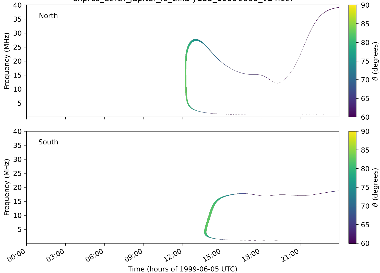
expres_earth_jupiter_io_txka-y235_19990605_v14.cdf
