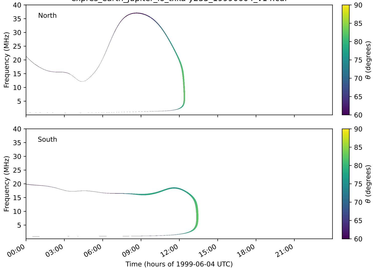
expres_earth_jupiter_io_txka-y235_19990604_v14.cdf
