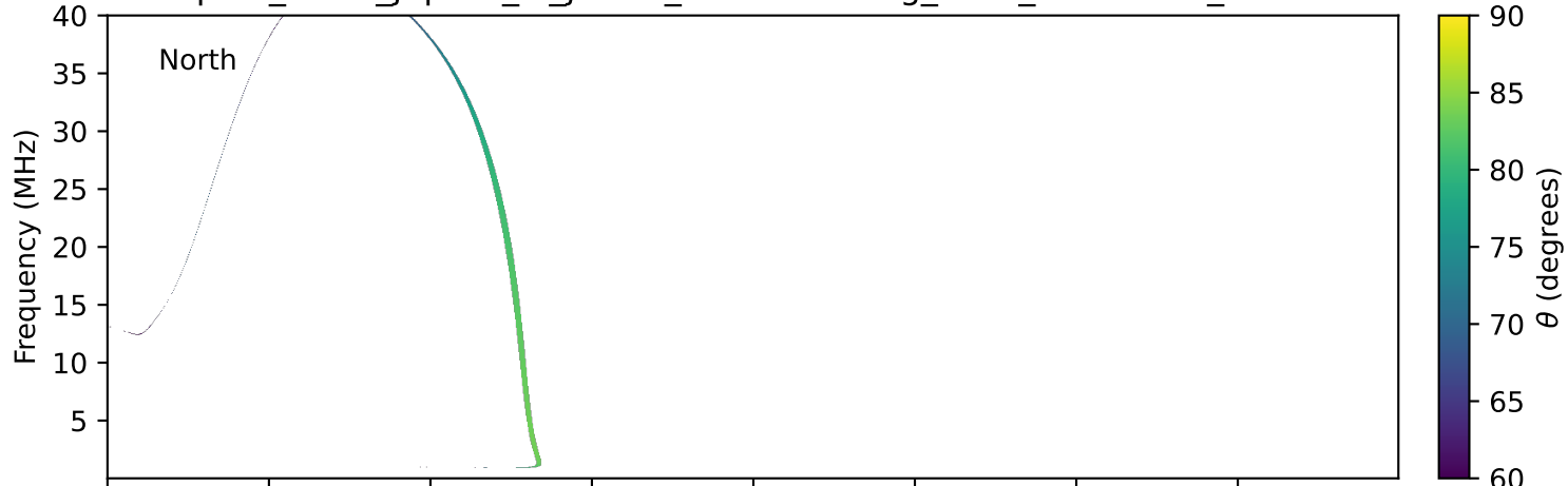
expres_earth_jupiter_io_jrm09_lossc-wid1deg_3kev_19990629_v11.cdf
