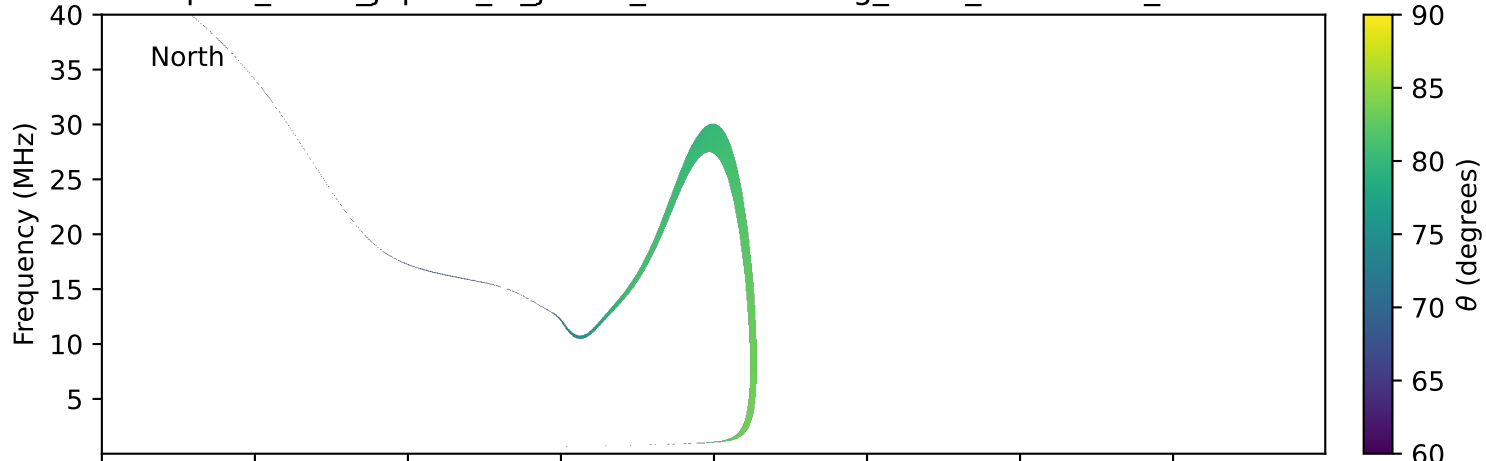
expres_earth_jupiter_io_jrm09_lossc-wid1deg_3kev_19990620_v11.cdf
